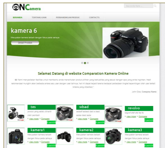
Gambar 7. Halaman Home
