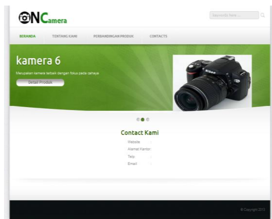
Gambar 9. Halaman Contact
